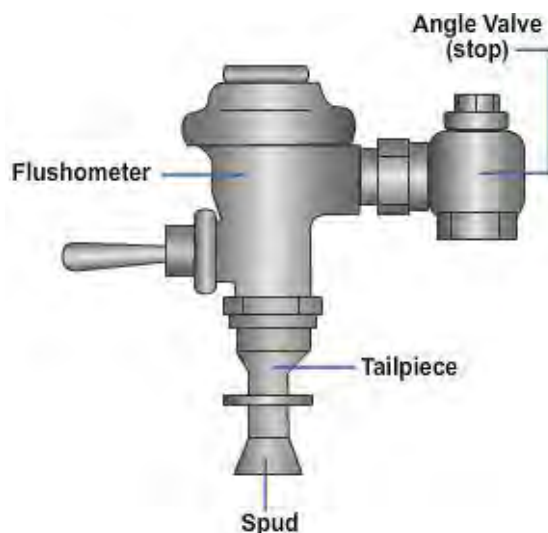
Figure 6-56 – Flushometer.
