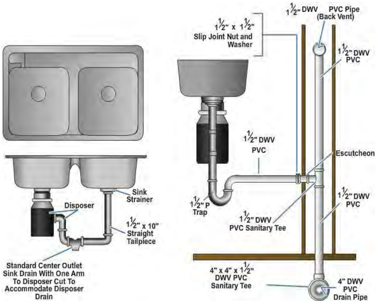
Figure 6-12 – Kitchen sink waste hookup.
